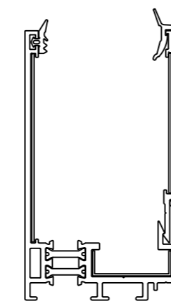
454001+492092/93 (493082 profile connector) (493006 profile connector) (493081 profile connector front plate)
