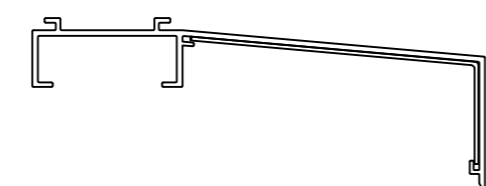
499080 for base profile 420031 (493086 profile connector)
