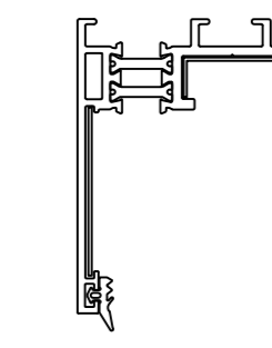
454012+492042/43 (493006 profile connector) (493034 profile connector)
