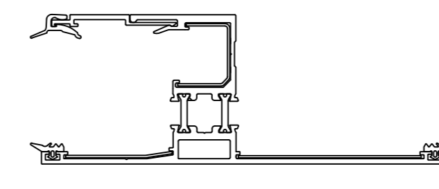
4440003+492042/43 (493011 profile connector) (493064 profile connector) (493063 profile connector)
