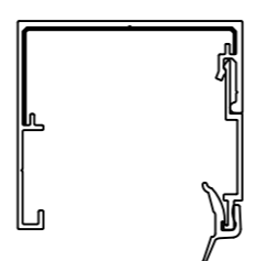
420040+492001 (493022 profile connector)
