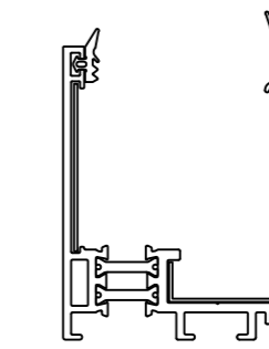
454011+492042/43 (493006 profile connector) (493034 profile connector)
