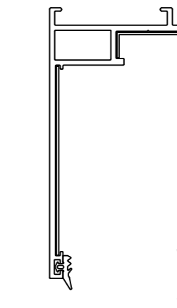
414002+492092/93 (493082 profile connector) (493006 profile connector) (493081 profile connector front plate)
