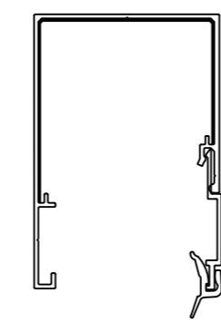
420080+492001 (493023 profile connector)
