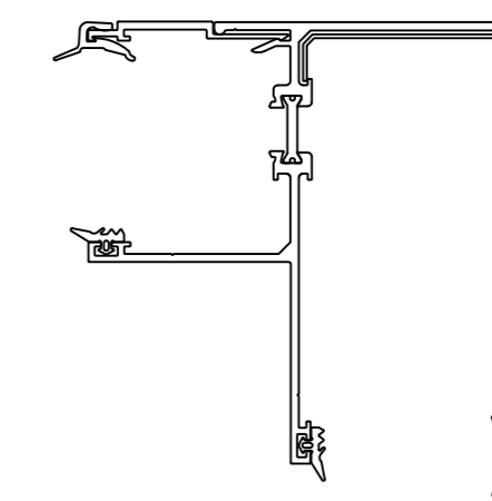
444072 + 2 x 492042/43 (493019 profile connector)
