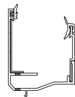
404051 + 492042/43 (493014 profile connector)
