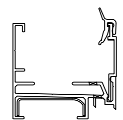
420031+492001 (493031 profile connector)
