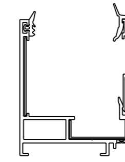
414011+492042/43 (493006 profile connector) (493034 profile connector)
